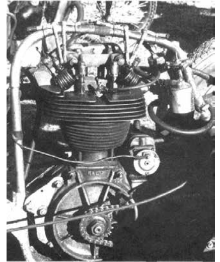
Above ES2 engine with stiffened drive-side crankcase. Below, early testing somewhere outside Sydney. Photos Graham Howard Collection.
